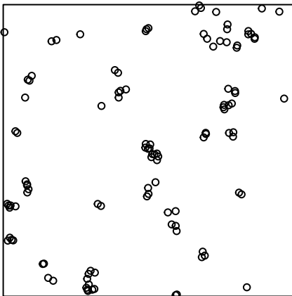
Clustered
