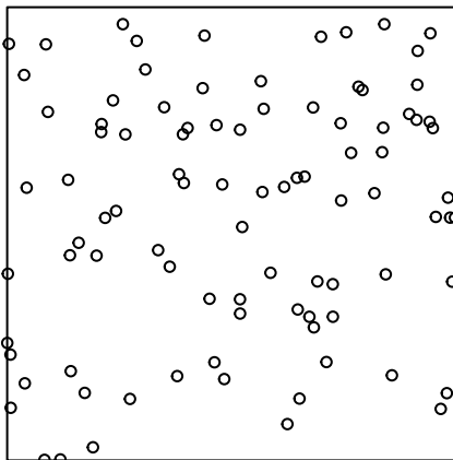
Independent
