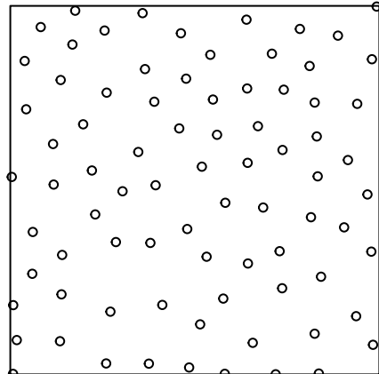
Regular
