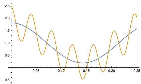
Figure 1: Weierstrass's Function
