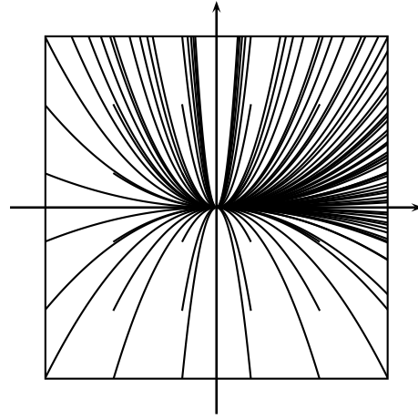
Figure 1: Two distinct real eigenvalues, same sign
