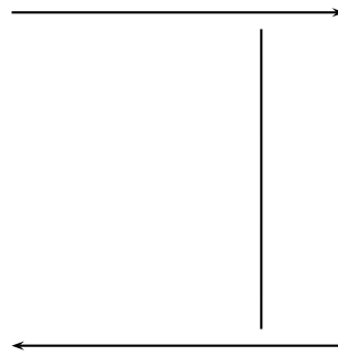
Figure 1: Reeb component
