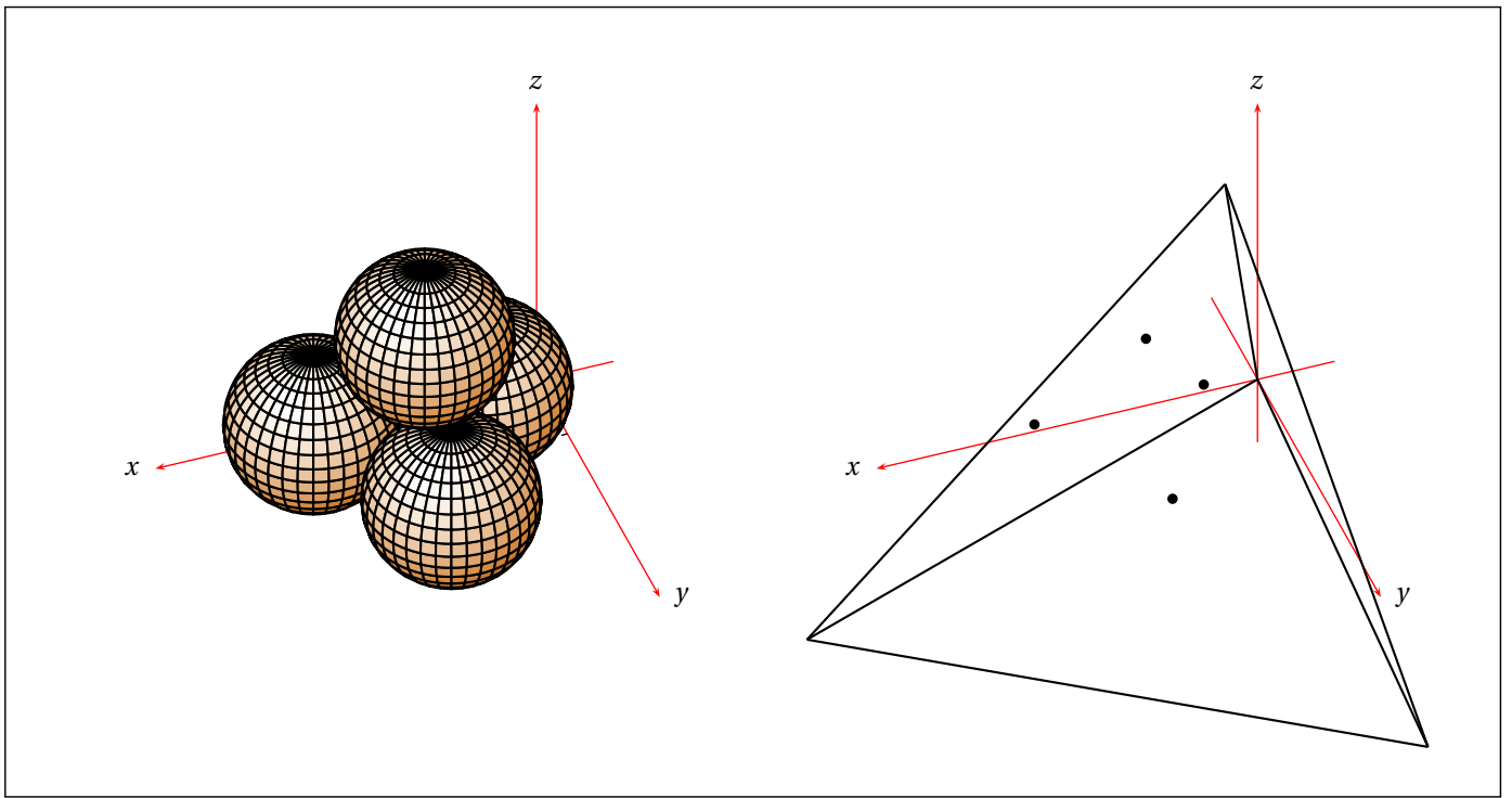
Figure 1: Four Spheres with Tetrad of Centers
