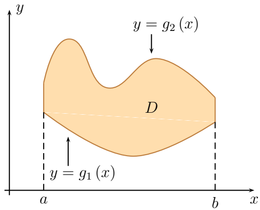
Figure 1: Integrals.
